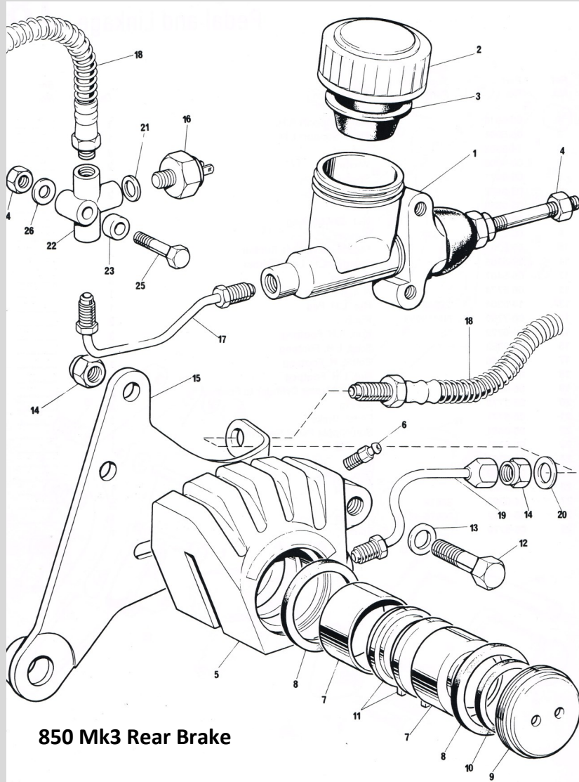
Fluid Reservoir, Master Cylinder
